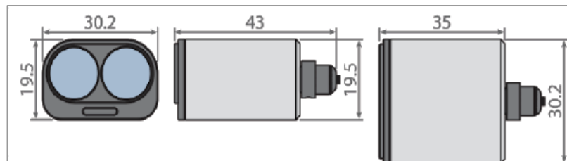
Figure 17: LW20/C dimensions
