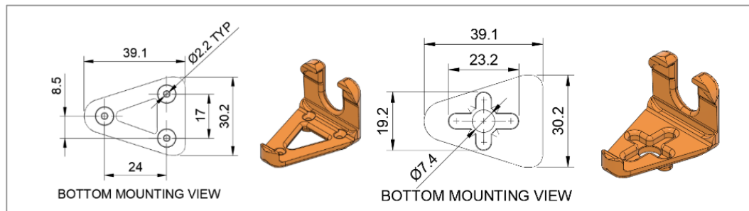
Figure 19: LW20/C mounting bracket options and dimensions
