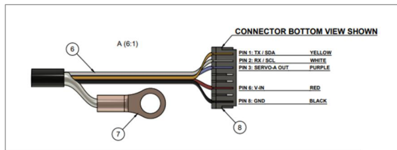
Figure 23: LW20/C communication pinout
